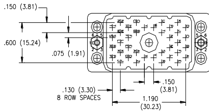
56 PIN PLUG
