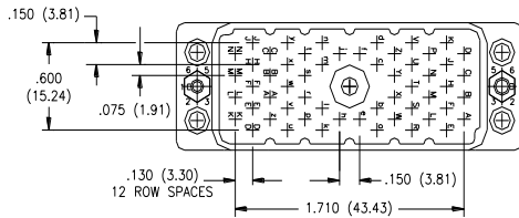
56 PIN PLUG
