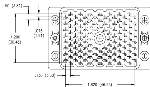
120 PIN PLUG
