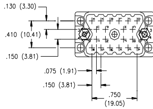
38 PIN PLUG
