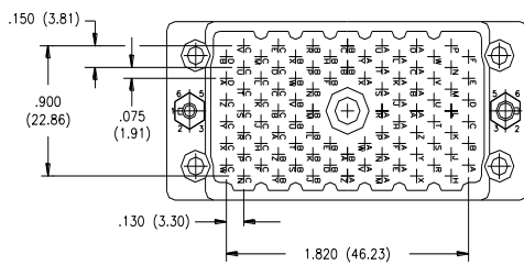
90 PIN PLUG
